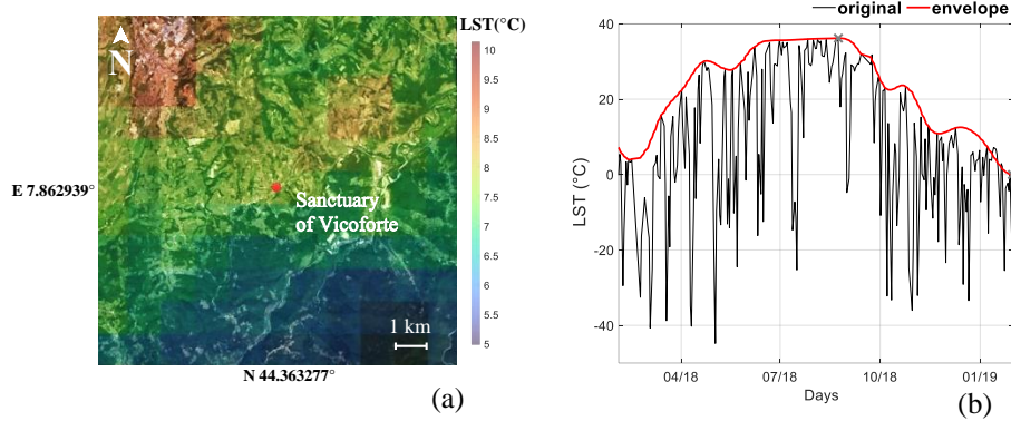
Fig. 1. Two-year (2018-19) average LST interpolated on the 11 km x 11 km grid around the Sanctuary superimposed on Google Earth view (a); LST time series: original and enveloped signal for S3A (morning) in 2018 (b).
