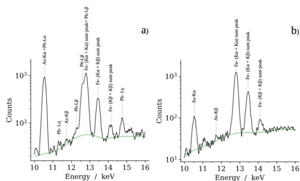
Figure 3. Comparison of two spectra acquired on different pulleys: on the left, the spectrum corresponding to 'Pulley 6', where lead and arsenic are present; on the right, spectrum acquired on one of the remaining pulleys, characterized by the presence of arsenic but not lead. Only the energy interval from 10 keV to 16 keV is reported. The black line is the acquired spectrum, while the computed baseline is in green.
