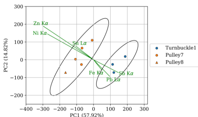
Figure 8. Score and loading plot of the first two components (PC1-PC2) calculated from XRF spectra acquired on bronze components. Percent variance captured by each PC is reported in parenthesis along each axis.
