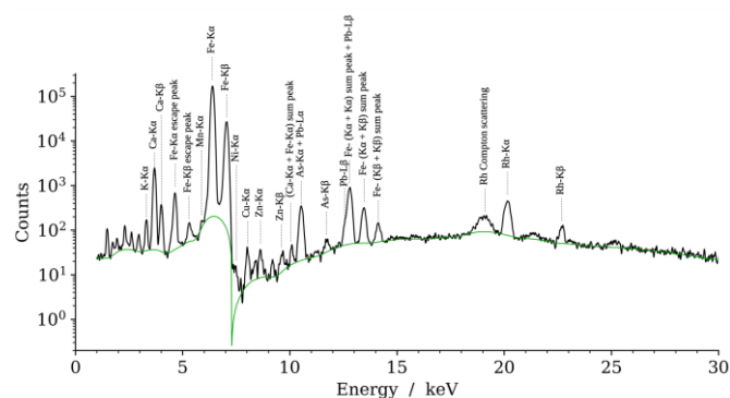
Figure 6. XRF spectrum acquired on one of the three-legged lewises. The black line is the acquired spectrum, while the computed baseline is in green.
