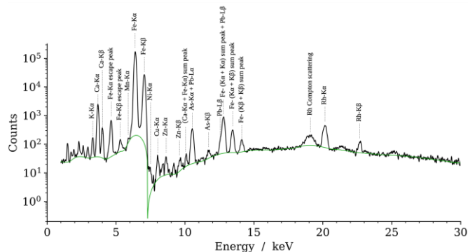
Figure 6. XRF spectrum acquired on one of the three-legged lewis. The black line is the acquired spectrum, while the computed baseline is in green.
