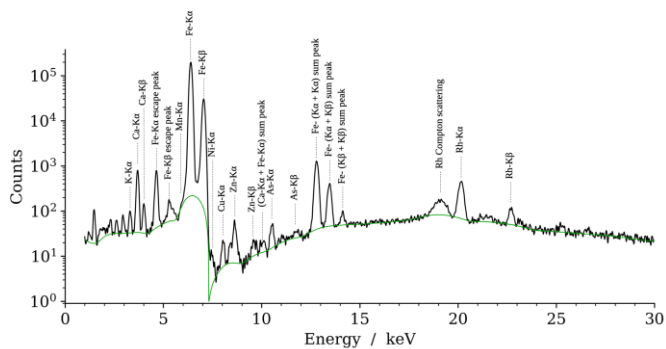
Figure 5. XRF spectrum acquired on the pincers. The black line is the acquired spectrum, while the computed baseline is in green.
