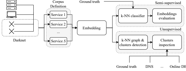
Figure 4: DarkVec overview.
