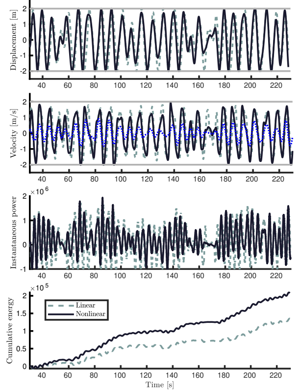
Fig. 7: Displacement, velocity, instantaneous power, and cumulative energy for an irregular wave realisation, for both linear (dashed-gray) and nonlinear (solid-black) moment-based controllers. The (scaled) wave excitation input is denoted using a dotted-blue line.
