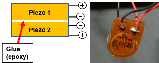
FIGURE 12: SCHEME OF THE SPECIAL TEST (LEFT), DETAIL PICTURE OF THE PIEZO JOINING (RIGHT)
