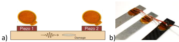
FIGURE 1: a) PIEZOELECTRIC COUPLE WORKING ON A DAMAGED STRUCTURE, b) EXAMPLE OF PIEZO GLUED ON SPECIMENS MADE OF THREE MATERIALS
