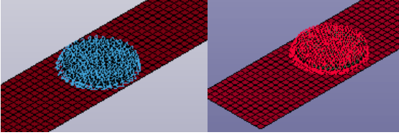
FIGURE 10: DETAILS OF BEAM MODEL: PIEZO 1 ACTUATOR (LEFT) AND PIEZO 2 SENSOR (RIGHT)
