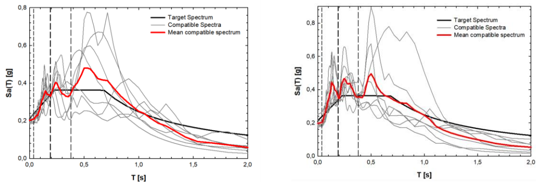
Fig. 9 - Input spectra at collapse: (a) x and (b) y direction
