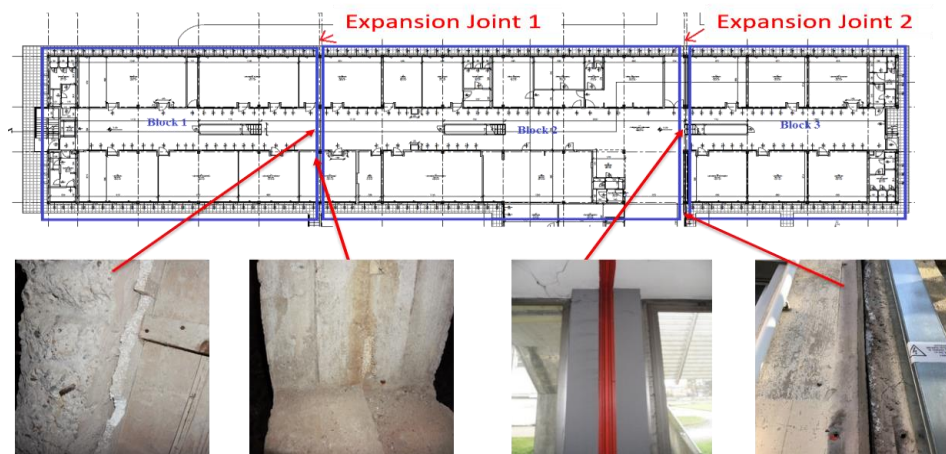
Fig. 2 - Expansion joints filled with polystyrene material
