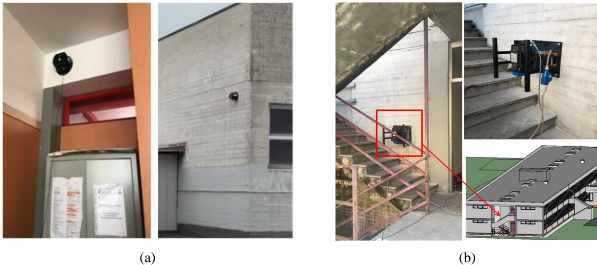
Fig. 4 – Installation examples of MEMS accelerometers (a) and vibrodyne positioning on the shear wall (b)
