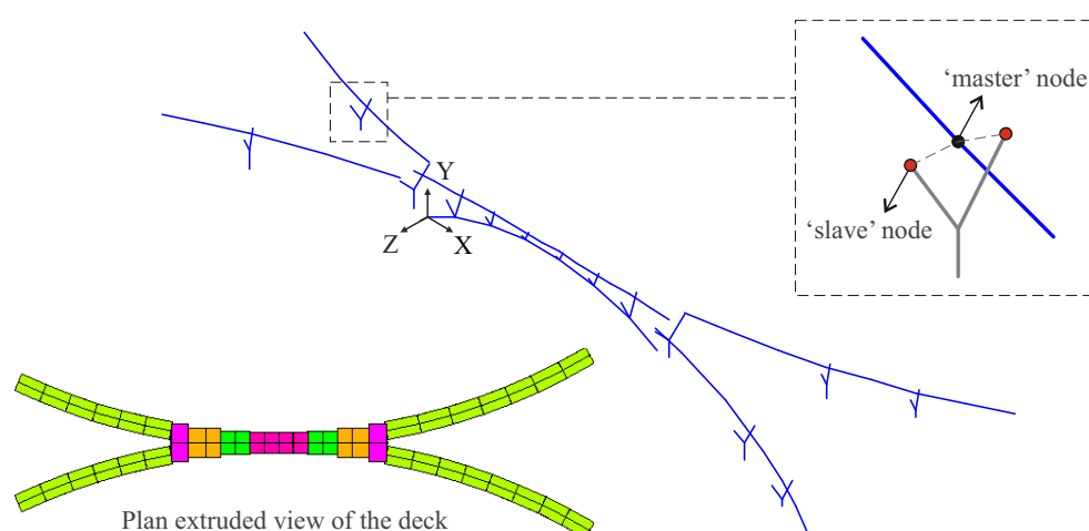
Figure 5. B model, with zoom on the pier–deck connection and deck cross sections.
