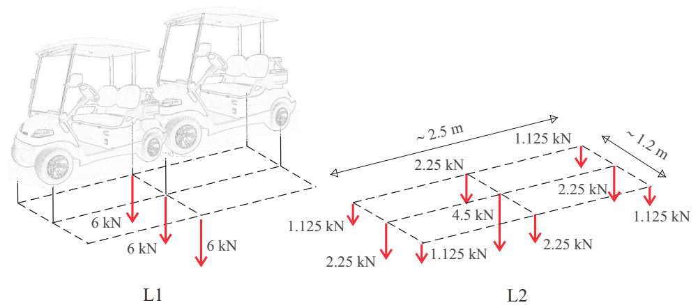
Figure 7. Scheme of load conditions L1 and L2 on S model.
