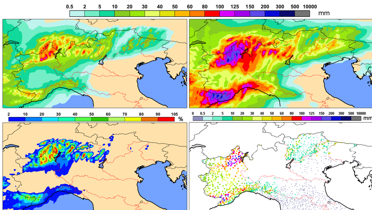
FIGURE 3 Italian Flash Floods products example with initialization on 2 October 2020 at 00 UTC and valid at 21 UTC the same day. The plots represent the 50th percentile (top left), the 99th percentile (top right), the probabilities of 6 h precipitation greater than 50 mm (bottom left) and the corresponding observations available in the MISTRAL portal for the same period (bottom right)
