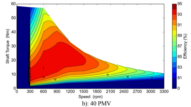
Fig. 12. Efficiency maps of the studied SPMand verneir machines.
