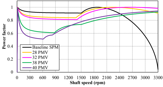
Fig. 8. Power factor vs. speed along the MTPA trajectory.
