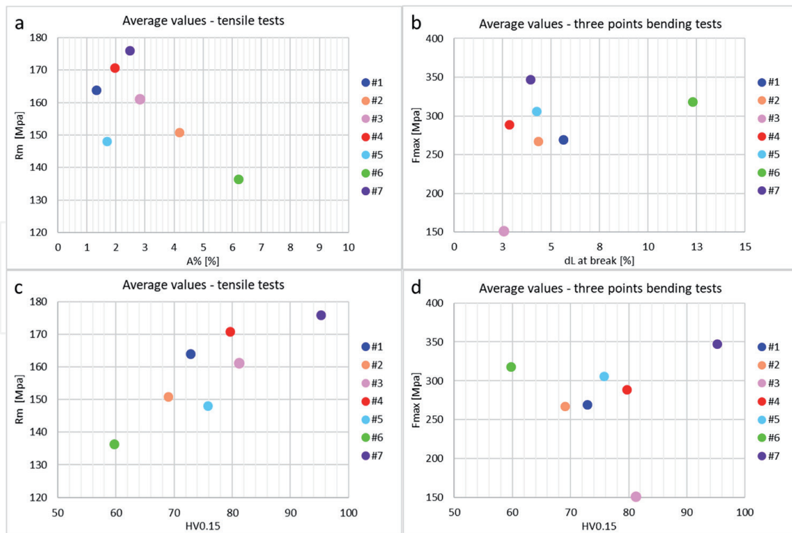
Figure 13. Average values from Tables 3 and 4. a: Average values R_m and A\% obtained after tensile tests. b: Average values F_{max} and dL\% obtained after bending tests. c: Average values HV_{0.15} and R_m obtained after tensile tests and microhardness measurements. d: Average values HV_{0.15} and F_{max} obtained after bending tests and microhardness measurements. FGM, FGM with Zn addition in EN AC 47000 and FGM with Zn addition in both alloys indicated as #1, #2, #3, while EN AC 47000 + Zn, EN AC 51100 + Zn, EN AC 47000, EN AC 51100 indicated as #4, #5, #6, #7.
