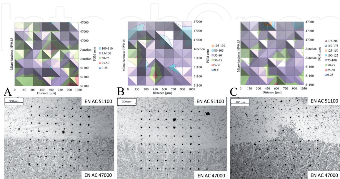
Figure 10. Microhardness maps for FGMS. A: FGM; B: FGM with Zn addition in EN AC 47000; C: FGM with Zn addition in both alloys.
