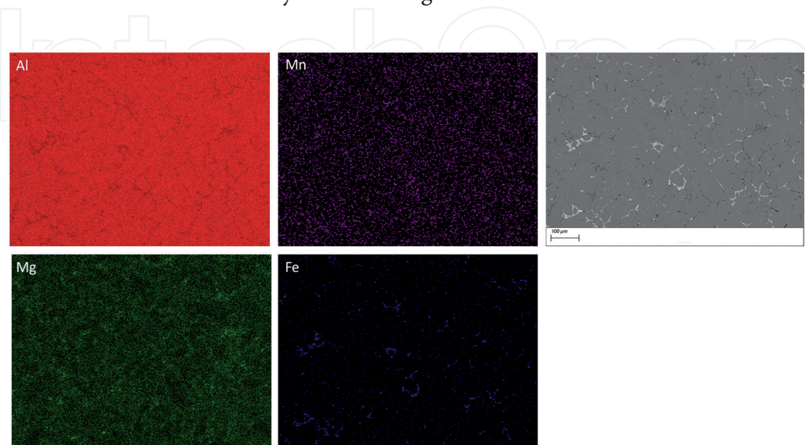
Figure 5. EDS maps analysis of EN AC 51100 bulk.
