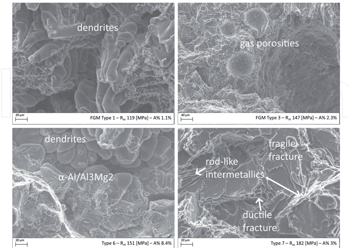
Figure 12. Fracture details. FGM type 1 is the FGM without Zn; FGM type 3 indicates the FGM with Zn in both compositions; types 6 and 7 are alloys EN AC 51100 and EN AC 47000 without Zn.
