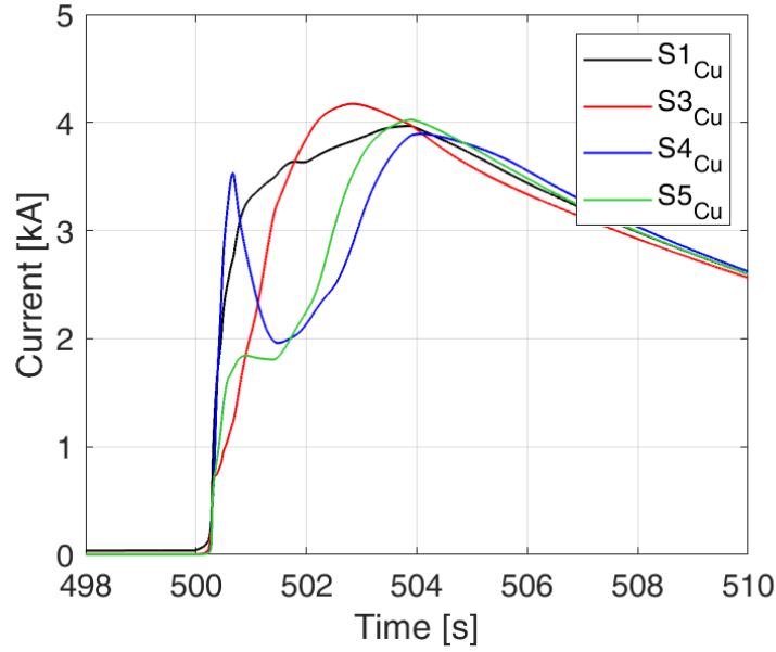
Figure 5.35: Evolution of the current in the copper profiles of selected strands in the interval around the quench detection and current dump.
