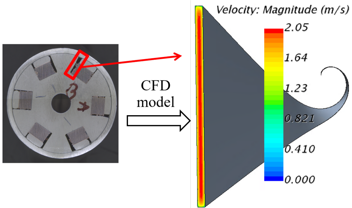
Figure 5.5: 3D Computational Fluid Dynamics model of the (twisted) sub-channel of the HTS ENEA CICC. The 2D distribution of the velocity is also shown.
