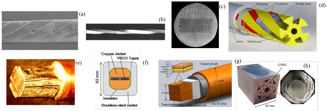
Figure 1.1: Concepts of HTS CICC and strands: (a) assembled cable based on Roebel idea (RACC), reproduced from [4], (b) Twisted and Stacked Tape Cable (TSTC), reproduced from [6], (c) Round Soldered and Twisted Stacked (RSTS), reproduced from [7], (d) Aluminum Slotted-Core Cable-In-Conduit Conductor, reproduced from [8], (e) Cross-Conductor (CroCo), reproduced from [13], (f) Stacked-Tapes Assembled in Rigid Structure (STARS), reproduced from [10], (g) Quasi Isotropic (QI) strand, [11] and (h) Conductor On Round Core (CORC), reproduced from [12]
