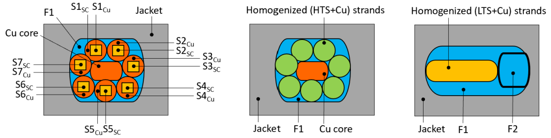
Figure 5.24: Discretization of the cross-section of the three layers (L1 to L3, from left to right) of the EU DEMO CS adopted in the H4C model.
