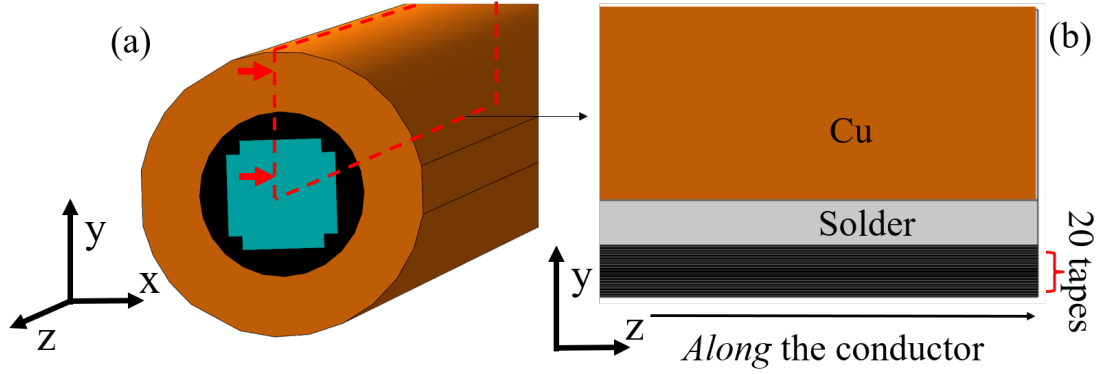
Figure 2.7: 3D view of the HTS CroCo strand (a) and 2D equivalent computational domain used for the 2D electro-thermal analysis (b).
