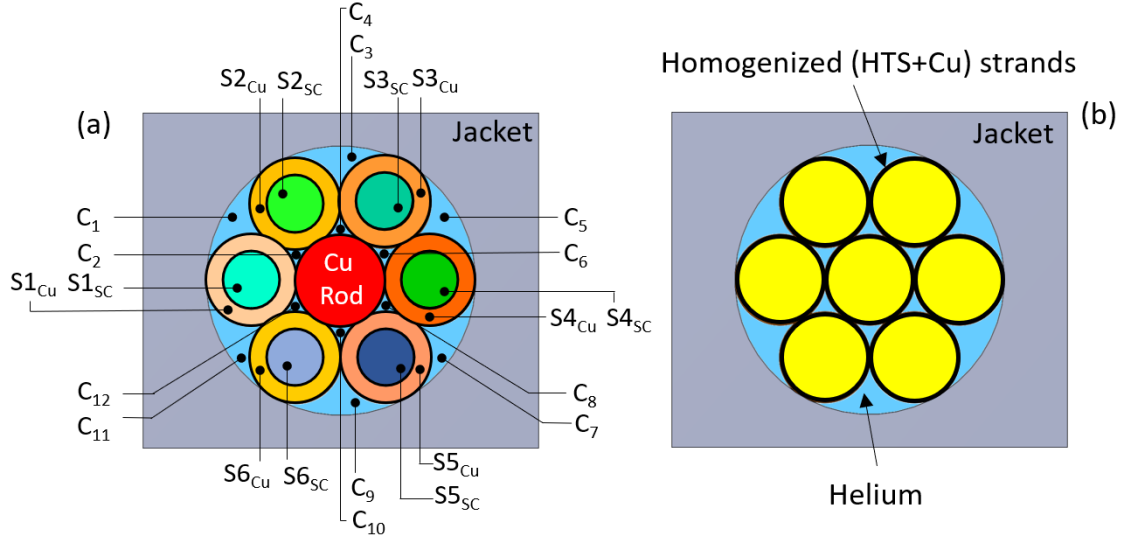
Figure 5.19: H4C (a) and 4C (b) cross-section discretization adopted for the HTS CroCo CICC. In (a), the distinction of the different thermal, electric (S#, with sub-regions SC and Cu) and fluid (C#) regions is shown.
