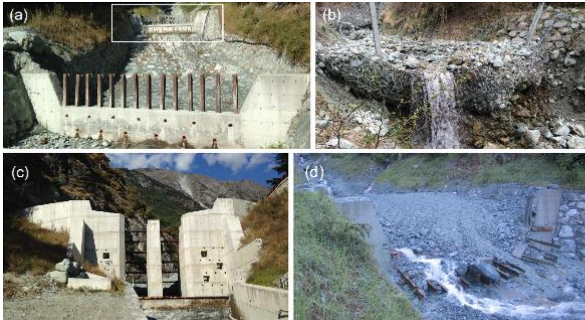
Fig. 2 The structural mitigation works along the Grand Valey torrent: (a) the two filter barriers at the Pèrriere hamlet; (b) the steel net barriers; (c) the slit-filter barrier at Tromen; (d) the barrier at Pèrriere (white rectangle in Fig. 2a) that collapsed in 2014. The position of each of these structures is indicated in Fig. 1 (photos courtesy of the Aosta Valley Autonomous Region).
