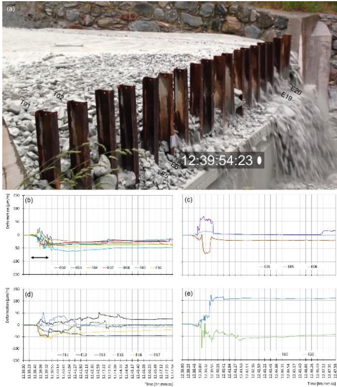
Fig. 9 Strain measurements recordings for the event on 9 June. (a) distribution of the deposit upstream of the monitored barrier; (b) and (c) data collected from E01 to E10 (i.e. the right side of the barrier), while (d) and (e) concern data from E11 to E20 (i.e. the left side of the barrier). The horizontal black arrow indicates the time interval in which compression (negative strain) increases.
