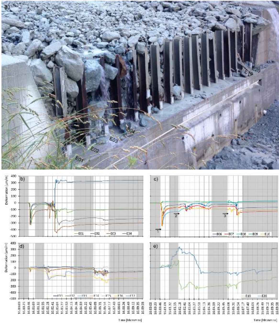
Fig. 10 Strain measurements for the event on 11 July. (a) distribution of the deposit; (b) and (c) collected from E01 to E10 (i.e. the right side of the barrier), while (d) and (e) concern data from E11 to E20 (i.e. the left side of the barrier). The black arrows in (c) give a rough indication of the initiation of each flow surge. The shaded areas indicate the time interval in which the measured strain remain roughly constant.
