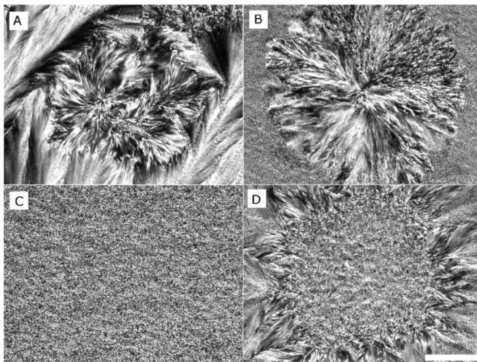
Fig. 4. Polarised light micrographs of CB (A), shea stearin and palm mid-fraction CBE, (B), CB and CBE 85:15 w/w mixture (C), and shea stearin and palm mid-fraction in a 60:40 w/w non-interesterified mixture (D). Bar represents 20 \mu\text{m} . Adapted from (Ghazani and Marangoni, 2018).
