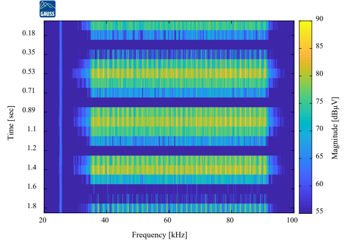
Fig. 4. Spectrogram of the G3-PLC signal
