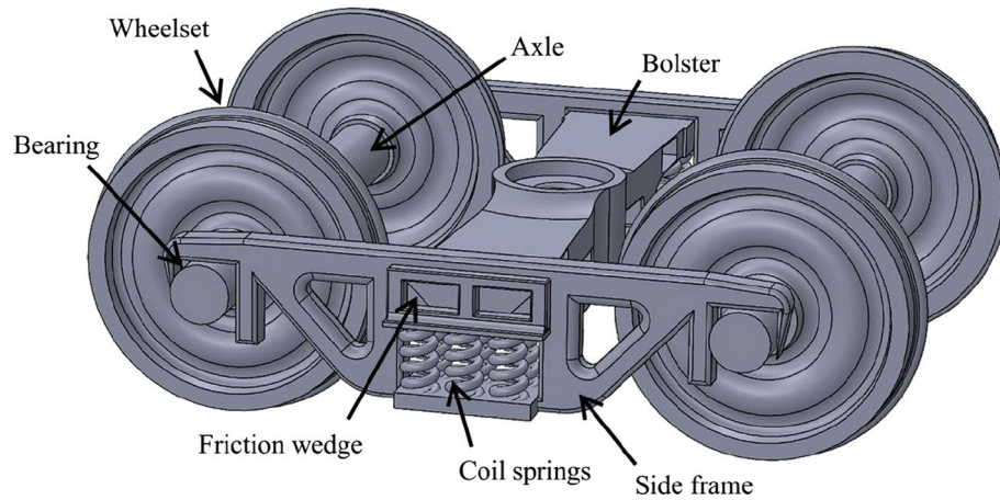
Fig. 1 Three-piece bogie
