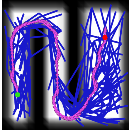
Fig. 8 Example of trajectory computed with the MP-RRT # by constructing a graph with 400 vertices. The start and target positions are in green and in red, respectively. In blue the graph \mathcal{G}^V in the reference space, while in magenta the computed path obtained from the graph \mathcal{G}^X in the state space.
