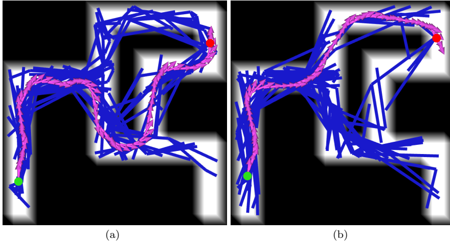
Fig. 7 Trajectories computed with the MP-RRT # by constructing a graph with 400 vertices. The start and target positions are in green and in red, respectively. In blue, the graph \mathcal{G}^V in the reference space, while in magenta, the computed path obtained from the graph \mathcal{G}^X in the state space. In (a) and (b) the target is in a similar position, but with opposite orientation. As a consequence, the solution is completely different, yielding different paths.
