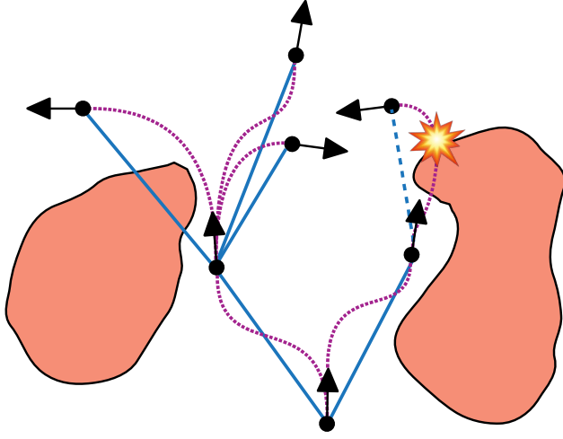
Fig. 1 Example of graphs constructed with MP-RRT#. The graph \mathcal{G}^Y consists of vertices (in black) and edges (in blue) in the reference state. Instead, the graph \mathcal{G}^X consists of trajectories (in magenta) obtained through evaluating the edges of \mathcal{G}^Y using the MPC strategy. An edge of \mathcal{G}^Y is labeled as invalid if its corresponding trajectory in \mathcal{G}^X crosses an obstacle.
