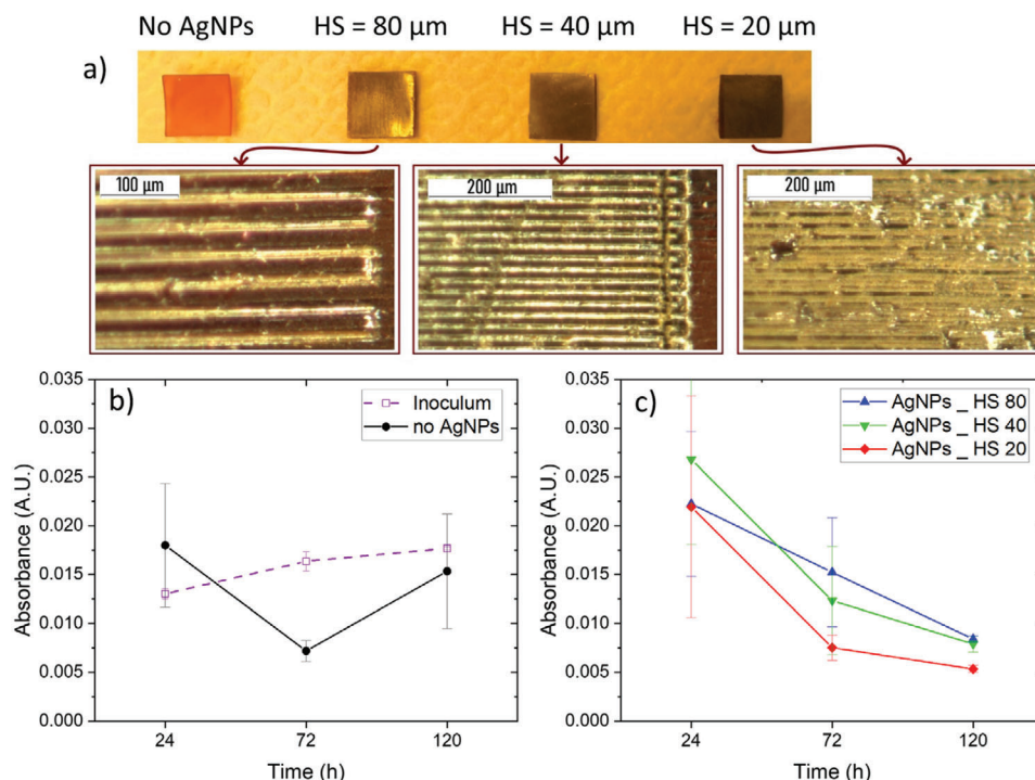
Figure 5. a) Pictures of the 3D-printed samples used for antibacterial tests showing the differences between the three hatch spacings (HS) of 80, 40, and 20 μm. Results from UV–vis analysis: b) absorbance values over time for the liquid solution containing only bacteria and medium (inoculum) in a 1:100 ratio and the same solution with the presence of 3D printed samples without silver nanoparticles generation (no AgNPs). c) Absorbance values over time for the bacteria solution containing: (i) 3D printed samples with silver nanoparticles generated with hatch spacing of 80 μm (AgNPs_HS 80), (ii) 3D printed samples with silver nanoparticles generated with hatch spacing of 40 μm (AgNPs_HS 40), (iii) 3D printed samples with silver nanoparticles generated with hatch spacing of 20 μm (AgNPs_HS 20).
