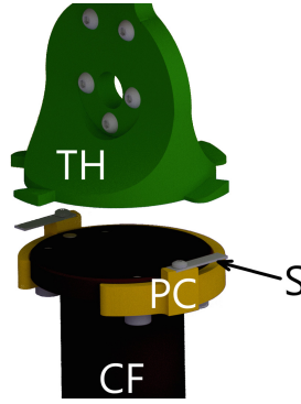
Fig. 5. The bayonet coupling between target-holder TH and the cold finger CF of the cryocooler. After lifting of CF to contact the base of TH, a 25° rotation engages one couple of TH wedges with the flexural springs S, bringing them in contact with the limiters on the positioning cup PC.
