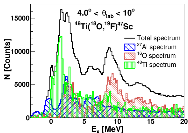
Figure 5. Decomposition of the excitation energy spectrum obtained with the \text{TiO}_2+^{27}\text{Al} target. The total spectrum is presented with the solid black line. The blue-hatched area corresponds to the normalized background originating from the ^{27}\text{Al} backing material, while the brown solid line corresponds to the background arising from oxygen. The green solid line is the obtained excitation energy spectrum for the ^{48}\text{Ti}(^{18}\text{O}, ^{19}\text{F})^{47}\text{Sc} reaction, after subtracting from the total spectrum the background contributions.
