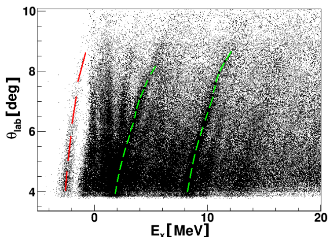
Figure 4. Bi-dimensional plot for the reconstructed scattering angle, \theta_{lab} , as a function of the excitation energy, E_x , for the data obtained with the \text{TiO}_2+^{27}\text{Al} target. The inclined loci, highlighted with the dashed-green and long-dashed red curves, correspond to the one-proton transfer reaction of ^{18}\text{O} with the oxygen and aluminum components of the target, respectively. The vertical loci correspond to the reconstructed events from the reaction on the ^{48}\text{Ti} target.
