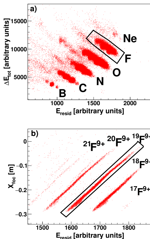
Figure 1. Typical particle identification spectra for the ^{48}\text{Ti}(^{18}\text{O},^{19}\text{F})^{47}\text{Sc} reaction at the energy of 275 MeV. a) \Delta E_{tot} as a function of the residual energy, E_{resid} , measured by one silicon detector of the FPD. A graphical selection of the fluorine ion events is illustrated by the solid black line. b) The horizontal position at the MAGNEX focal plane, X_{foc} , as a function of the residual energy gated by the selected fluorine ions of panel (a). The different loci correspond to ions with different \sqrt{m}/q . A graphical selection on the ^{19}\text{F}^{9+} events is shown by the solid black line.
