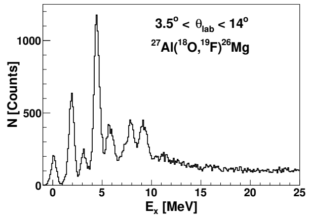
Figure 3. Reconstructed excitation energy spectrum for the ^{27}\text{Al}(^{18}\text{O}, ^{19}\text{F})^{26}\text{Mg} reaction at 275 MeV.
