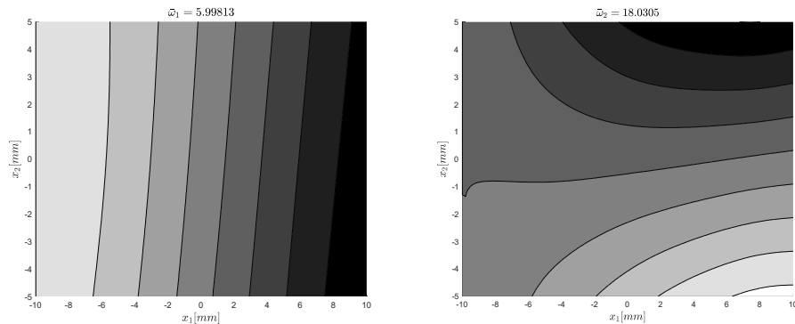
FIGURE 1. Modal shapes (flexural and torsional) for cantilever rectangular symmetric angle-ply sandwich plate ( h_c/h=8 ).
