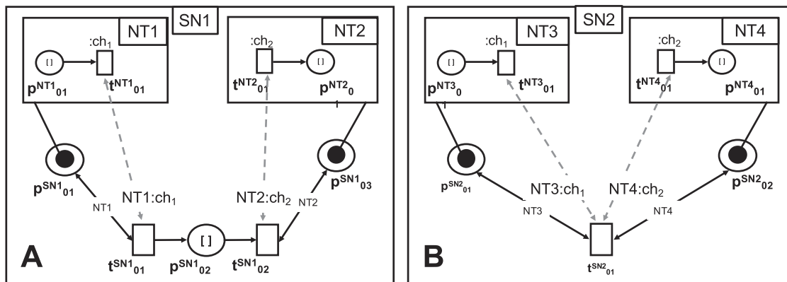
Fig. 7. NWN representation of the two signaling mechanisms relevant for modeling ontogenetic processes: (A) In paracrine signaling, the cell NT1 uses channel ch_1 to send a signal (black token) to the extracellular environment modeled as a place in the system-net ( p_{01}^{SN1} ). Cell NT2 that is in spatial proximity receives the signal using channel ch_2 . (B) In juxtacrine signaling, the two adjacent cells (NT3 and NT4) engage in direct communication through channels ch_1 and ch_2 .
