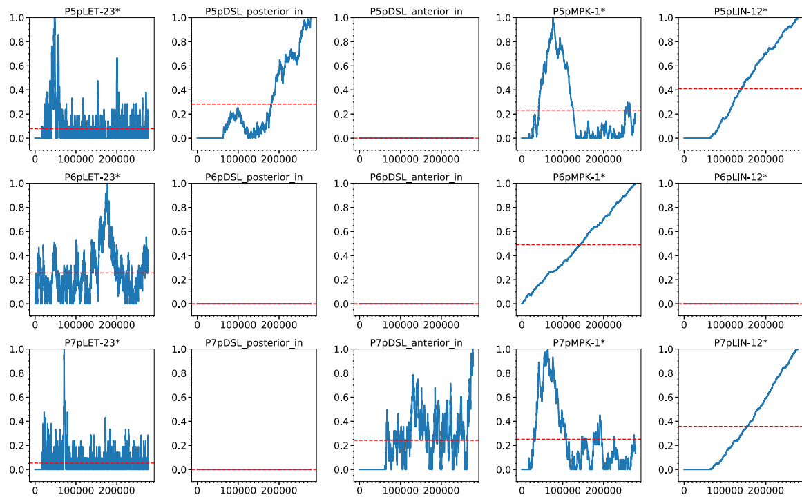
Fig. 17. P5.p, P6.p, and P7.p dynamic behavior. The dynamic marking evolution of relevant places along with the simulation in the Pn.p models correctly recapitulates physiology. P6.p (central row) receives strong LIN-3 signaling from the AC, resulting in strong LET-23 and MPK-1 activation and DSL-mediated lateral signaling to neighbors. P5.p and P7.p (top and bottom rows, respectively) receive weaker, delayed LIN-3 signal, inducing weak LET-23 activation, leading to moderate active MPK-1 levels, which are inhibited by the high LIN-12 activation induced by the DSL lateral signaling from the P6.p cell, inducing the Secondary fate.
