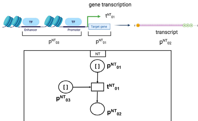
Fig. 32. Activating gene regulation. It models the positive regulation of a transcription process. This module includes a net-token place for the gene to be transcribed ( p_{01}^{NT} ), one for the transcription products ( p_{02}^{NT} ), and one for the regulatory signal (for example, a transcription factor) activating transcription ( p_{03}^{NT} ), while t_{01}^{NT} models the transcription process, which depends on the presence of the activating signal.
