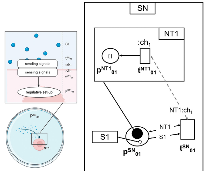
Fig. 26. Signal sensing. It models a cell sensing a signal from the extracellular environment. In this module, the net-token occupying a place in the ISG (NT1) senses the signal modeled with the colored token S1 in the same place p_{01}^{SN} it occupies via a communication channel:ch 1 , linking transitions t_{01}^{SN} in the system-net (SN) and t_{01}^{NT1} in NT1.
