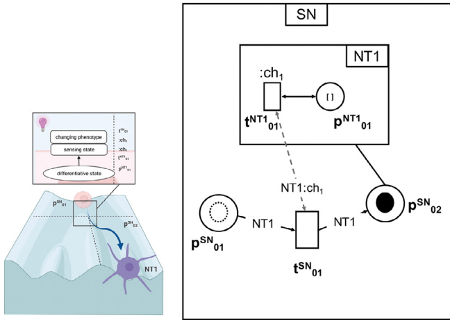
Fig. 28. Differentiative step. It models a cell changing its phenotypic state. This passage is regulated by a checkpoint evaluating the cell state. This module includes the net-token occupying a place in the DL (NT1 in p_{01}^{SN} ). If NT1 internal state activates the checkpoint in t_{01}^{SN} via a communication channel: ch_1 (linking t_{01}^{SN} in the system-net and t_{01}^{NT1} in NT1), the DL transition moves NT1 to p_{02}^{SN} , modeling the new phenotypic state.
