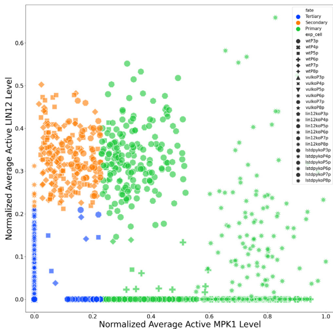
Fig. 19. Simulations results. This plot illustrates that simulations from different experimental conditions (wt, vul_ko, lin12_ko and lstdpy_ko) correctly recapitulate the expected biological behavior in terms of markers levels and assigned fates for the Pn.p cells.
