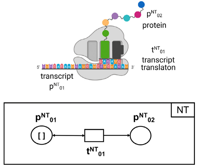
Fig. 30. Translation. It models the translation of an RNA transcript into a protein product. This module includes a net-token place for the RNA molecules to be translated ( p_{01}^{NT} ) and one for the translation products ( p_{02}^{NT} ), while t_{01}^{NT} models the translation process.
