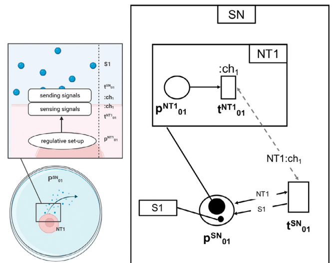
Fig. 27. Signal sending. It models a cell sending a signal to the extracellular environment. In this module the net-token NT1 sends the signal modeled with the colored token S1 in the same place it occupies in the ISG ( p_{01}^{SN} ) via a communication channel:ch 1 , linking transitions t_{01}^{SN} in the system-net (SN) and t_{01}^{NT1} in NT1.
