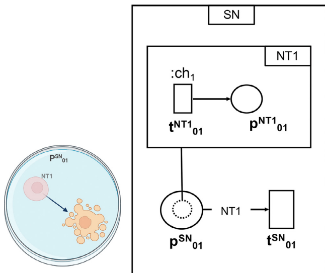
Fig. 25. Apoptosis. It models a cell undergoing apoptosis that leaves the position it occupied in the environment empty. This module includes the apoptotic cell (NT1) in a position in the ISG ( p_{01}^{SN} ) being removed from the ISG via a transition ( t_{01}^{SN} ) in the system-net (SN).
