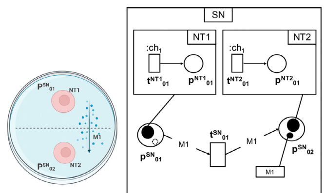
Fig. 23. Molecular flow. It models the mobility of a molecule from a one position to another one in the physical environment. This module models the movement of a colored token (M1) from a place in the ISG ( p_{01}^{SN} , holding the net-token NT1) to another one ( p_{02}^{SN} , holding the net-token NT2) via a transition ( t_{01}^{SN} ) in the system-net (SN).
