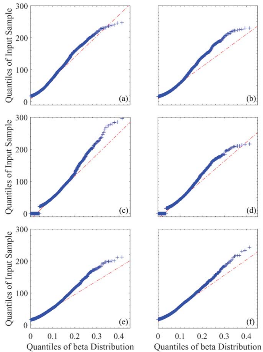
Figure A5. Q-Q plot for the resulting pore size distributions for each VISF test at 271 K considering a Beta distribution with \alpha = 1.2 and \beta = 15 . Tests on the left (a,c,e) are ON-shelf, while tests on the right (b,d,f) are OFF-shelf. (a,b) are for sucrose 5%, c and d are for mannitol 5% and e and f are for dextran 10%.
