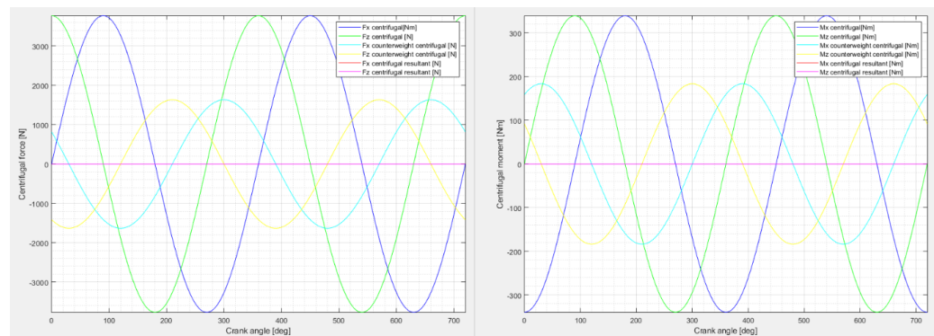
Figure 12. Centrifugal forces (left) and moments (right) for a 3 cylinder in-line engine.
