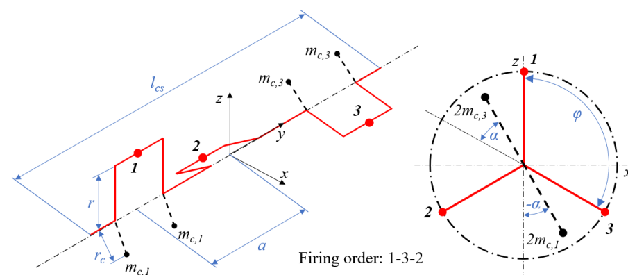
Figure 1. Model of the crankshaft for a 3 cylinder in-line engine, with the relative polar plot on the right.
