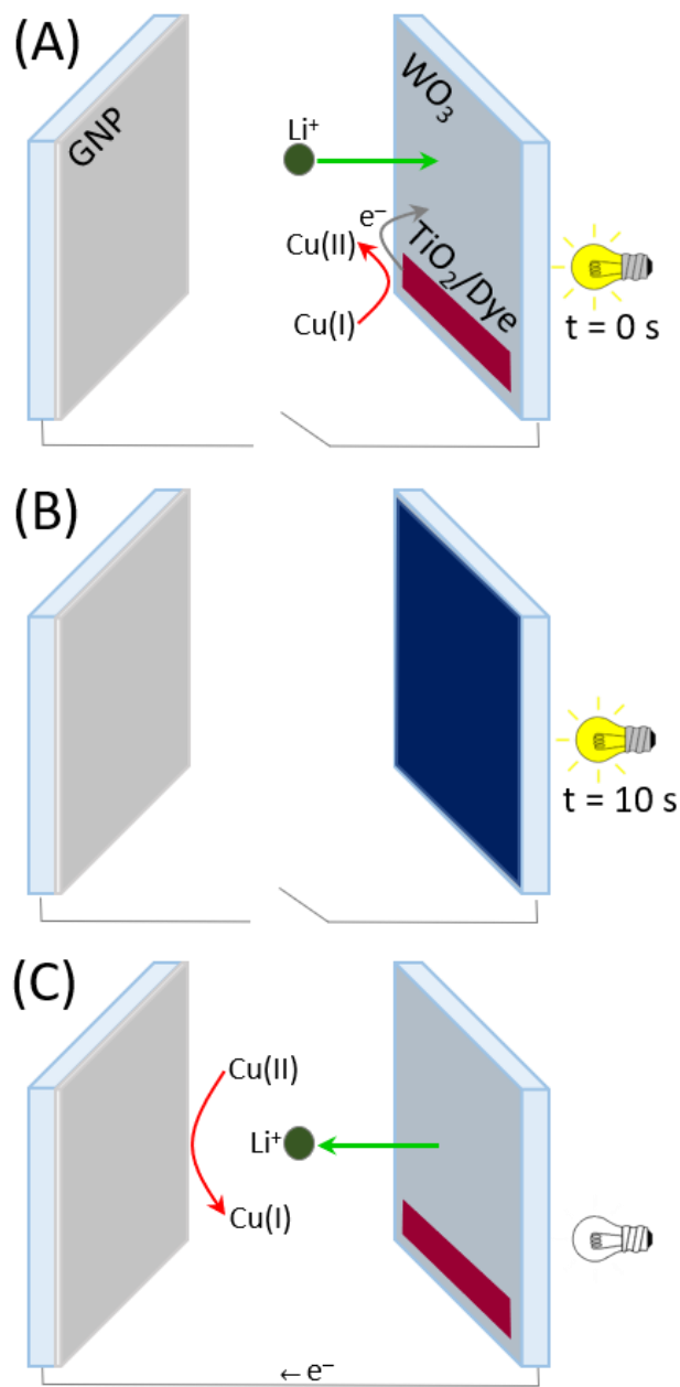
Fig. 2. Schematic diagram of the PECVD in: (A,B) open-circuit conditions under simulated sunlight (at t = 0 and after 10 s); (C) short-circuit under dark conditions. The oxidation and reduction of the Y123 dye is not drawn so as not to complicate the readability of panels (A) and (C).
