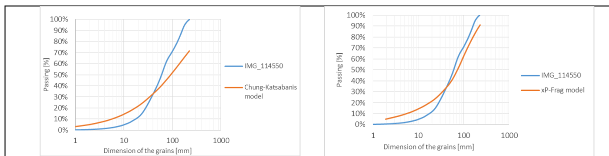
Figure 6. Left: Comparison between the particle size distributions obtained with Split Desktop and with the Chung-Kastabanis model and xP-Frag.
