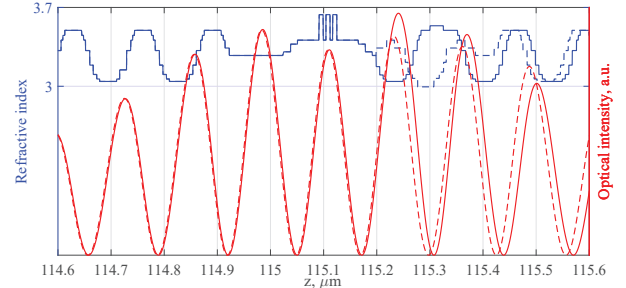
Fig. 1: Refractive index (in blue) and standing wave (in red, from VELM) for the two VCSELs: continuous lines - TJ; dashed - oxide confined. Ground contact is placed at z = 0 \mu\text{m} , output light is emitted at the right hand side ( \lambda = 847.7 \text{ nm} and G_{th} = 1480 \text{ cm}^{-1} for the TJ-VCSEL; \lambda = 847.9 \text{ nm} , G_{th} = 1440 \text{ cm}^{-1} for the oxide confined).
