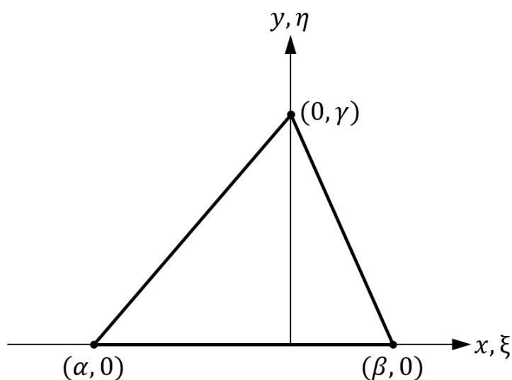
Figure 5. Local reference system for the contact formulation.
