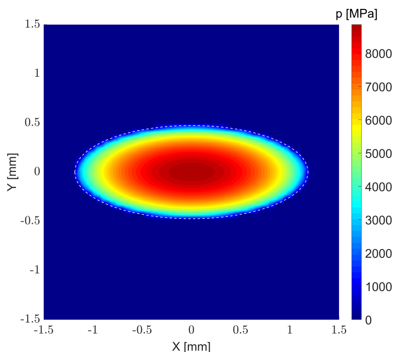
Figure 6. Pressure distribution for the ellipsoid–ellipsoid contact.
