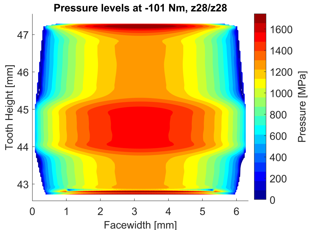
Figure 23. Flank pressure distribution of the tested gear pair with parabolic tip relief, dCa = 94.245 mm and Ca = 32 \mu\text{m} and C_\beta = C_{\beta In} = C_{\beta Fin} = 2 \mu\text{m} , zL = b/2 and zLc = 0.8b parabolic crowning.
