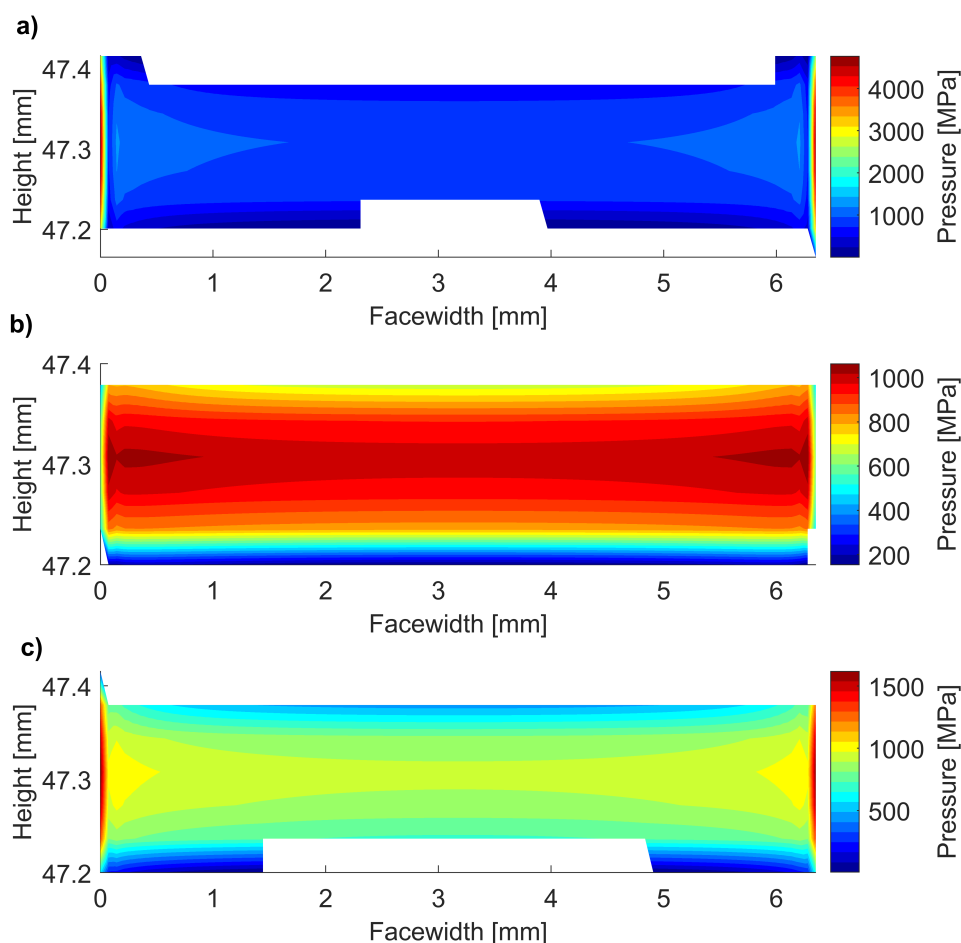
Figure 9. Effect of plane mirroring on the pressure distribution for meshing gears. (a) No mirroring, b_p = b_g (b) Mirroring, b_p = b_g (c) Mirroring, b_p = 2b_g .
