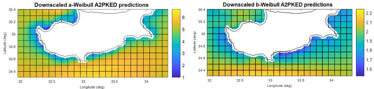
Figure 5. Downscaled a, and b-Weibull parameter estimation computed by ATPKED
