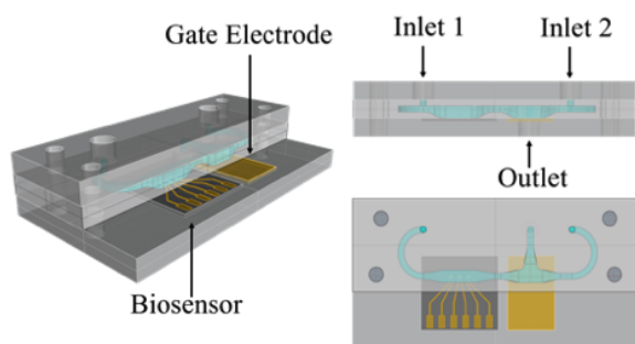
Figure 1. 3D model of the microfluidic platform.
