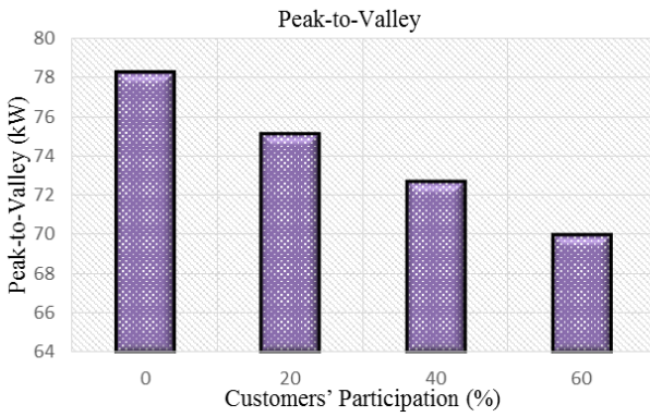
Fig 7: The amount of peak-to-valley of load curve in the base case with different customers' participation
