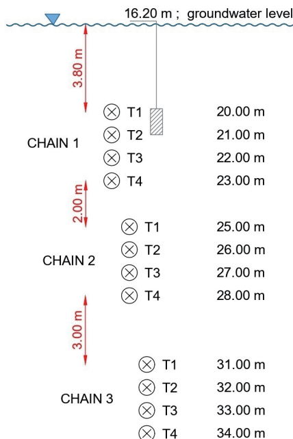
Fig. 4 - Simplified conceptual scheme of the water temperature measuring chain (PT1004/Pt) installed in S2-control piezometer of the Politecnico of Torino open-loop GWHPs
