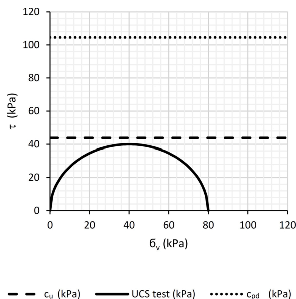
Fig. 15. UCS Mohr circle representation, c_u , and average of \tau_{\text{peak}} ( c_{\text{pd}} ) for the two-component grout cured for 1 hour.
