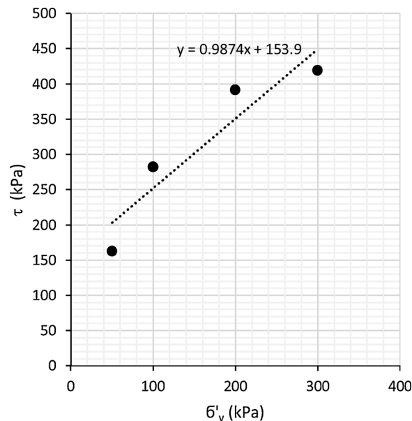
Fig. 10. Mohr-Coulomb failure criteria envelope pertaining to two-component grout samples cured for 24 h.
