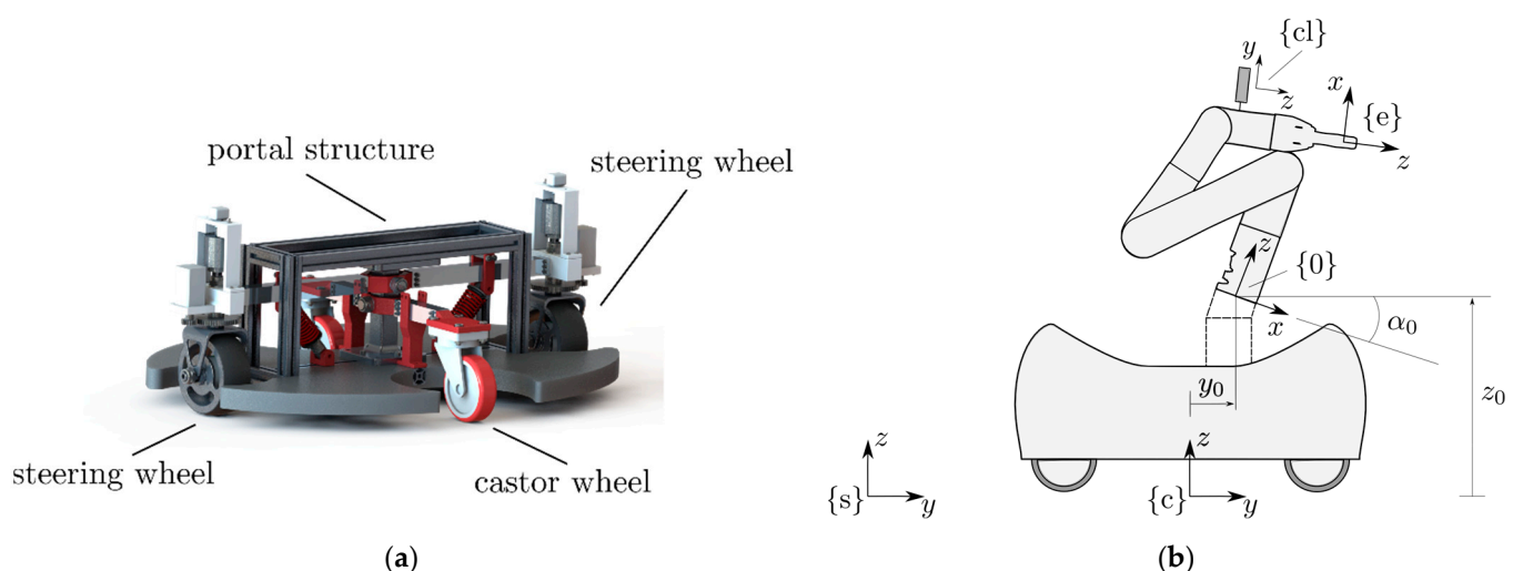
Figure 1. (a) The updated Paquitop mobile platform with the mounting structure. The two steering wheels are positioned along the major axis of the elliptical footprint, and the passive castor wheels are positioned along the minor axis. Thus, the resulting support polygon has a rhombic shape. (b) Paquitop.arm system and reference frame definition. Notice that \{c\} is fixed to the mobile platform, positioned at ground level and in the center of the elliptical footprint. \{cl\} is the r.f. of a LiDAR camera, which is presented and discussed below.
