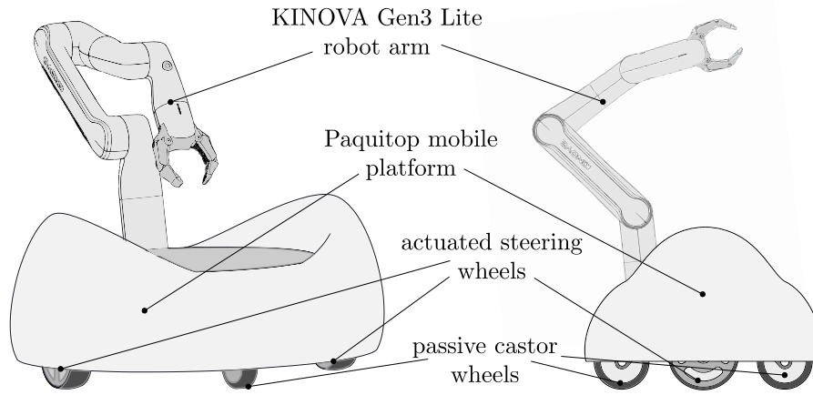
Fig. 1. The Paquitop mobile platform provided with the six degrees of freedom KINOVA Gen3 Lite collaborative manipulator.
