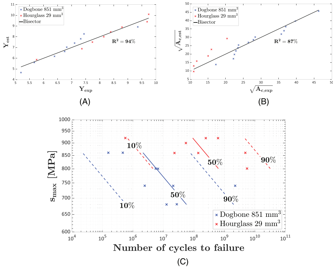
FIGURE 11 Fitting capabilities of the proposed approach for heat C specimens in Furuya 36 : (A) Q-Q plot for the VHCF life; (B) Q-Q plot for the critical defect size; (C) S-N plot of experimental data and estimated P-S-N curves for dog-bone and hourglass specimens [Colour figure can be viewed at wileyonlinelibrary.com ]
