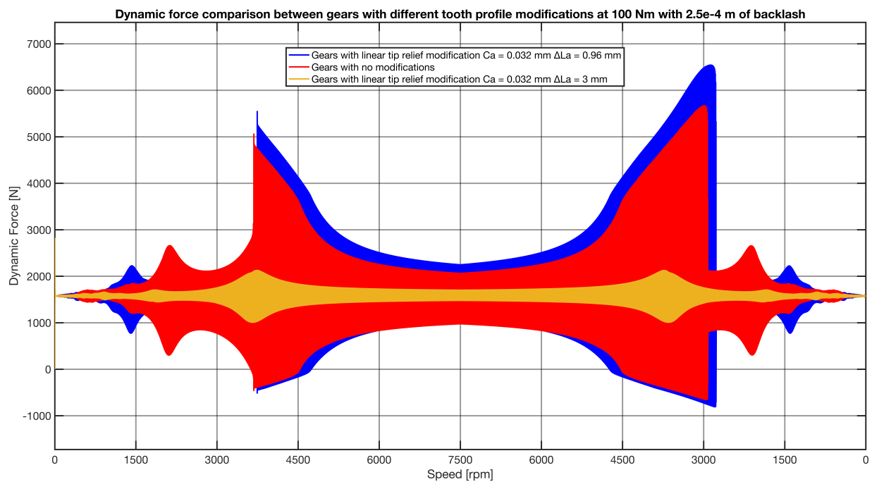
Figure 11. Comparison of the Dynamic Force of the gearset at different profile modification.
