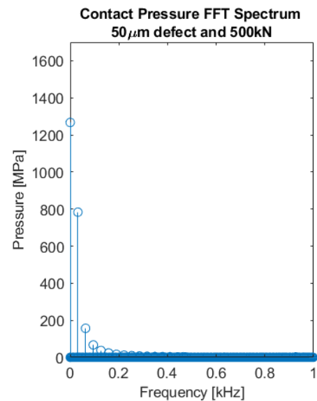
Figure 7. Harmonic content of a time history.
