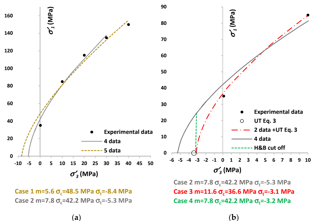
Figure 2. (a) Comparison of data fitting of triaxial compression tests of Vosges sandstone with a confinement range \sigma'_3 = 0.1 –40 MPa and \sigma'_3 = 0.1 –30 MPa. (b) Comparison of data fitting with confinement range \sigma'_3 = 0.1 –30 MPa (grey line) and \sigma'_3 = -3.4 –10 MPa (red line). The open symbol, UT Equation (3), is the uniaxial tensile strength estimated with Equation (3). The green line is the tensile cut off calculated with \sigma_c/\sigma_t = 0.81m + 7 .
