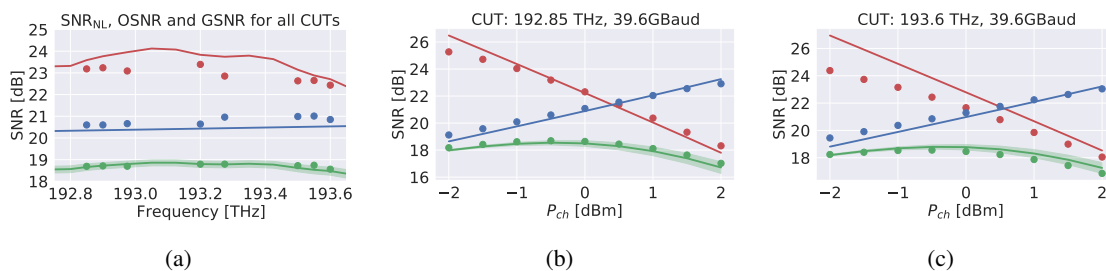
Fig. 3: (a) The measured and simulated SNR NL , OSNR and GSNR values for all CUTs in the optimal input power per channel scenario (-0.5 dBm). (b), (c) Power sweeps for two selected channels. For all plots, the red, blue and green circles are the SNR NL , OSNR and GSNR values as measured from the OSA at the line termination; the coloured lines show the respective simulated GNPpy values. The shaded area surrounding the green solid lines represents the variation of the GSNR prediction varying the connector loss within a 0.5 dB range.
