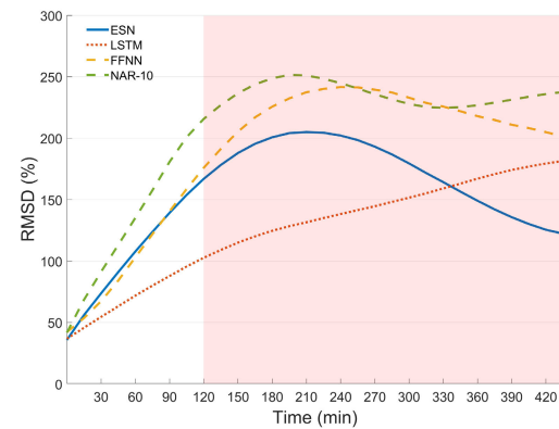
(c) RMSD
