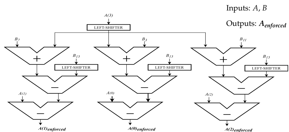
Figure 2. Enforcement architecture.
