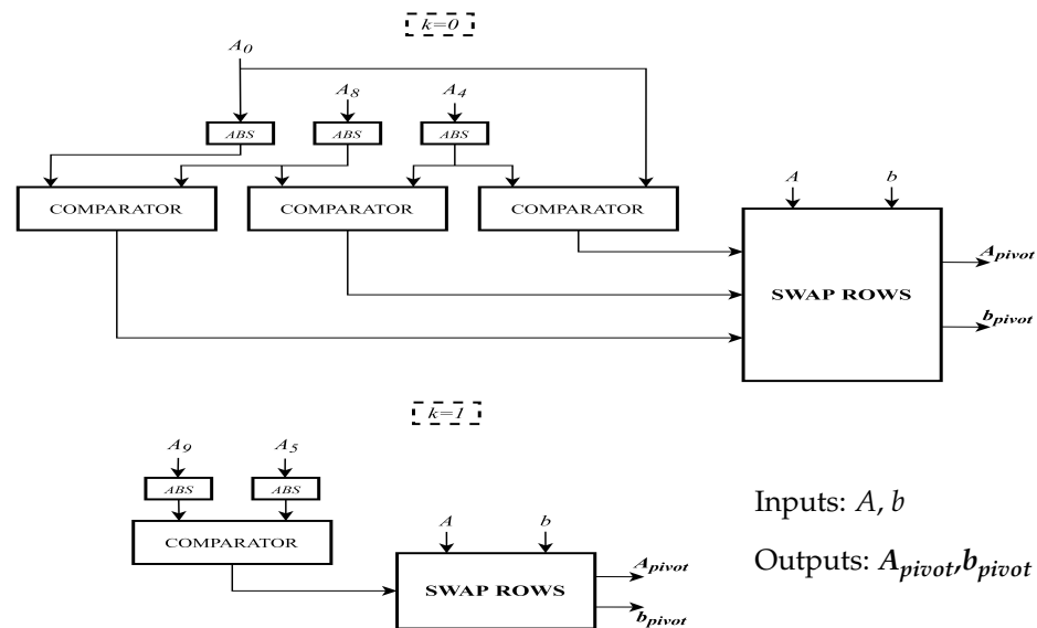
Figure 3. Partial Pivoting architecture.
