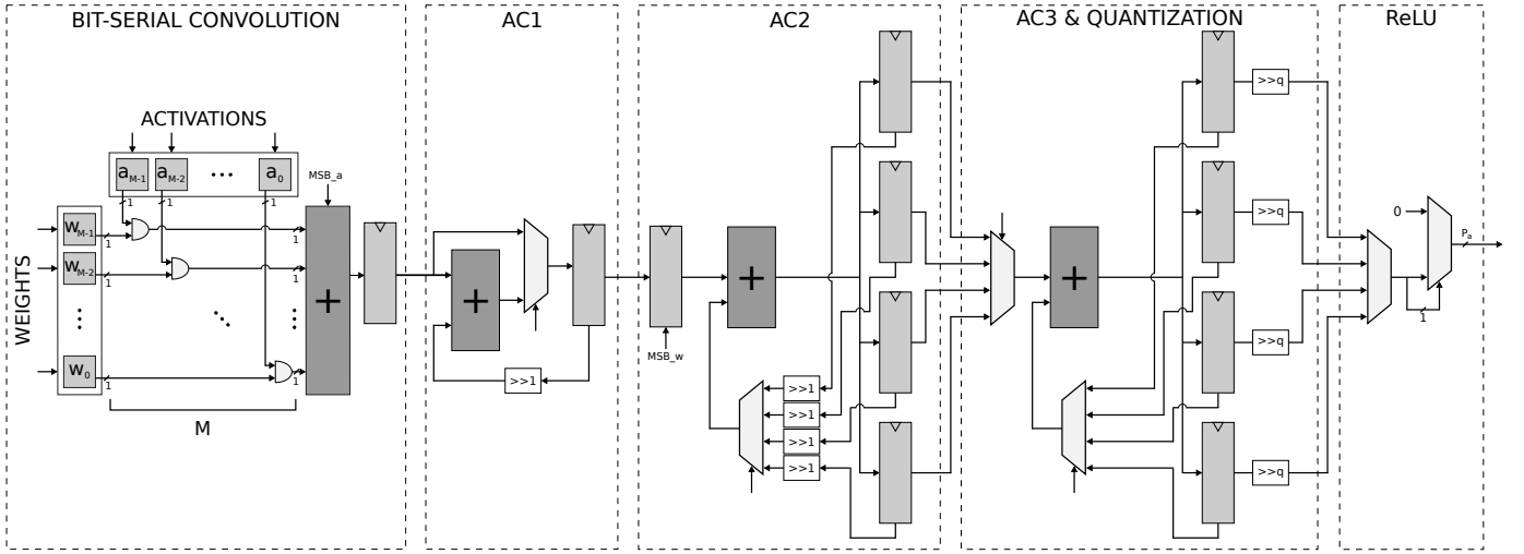
Fig. 2. Datapath architecture of a single SMAC block.
