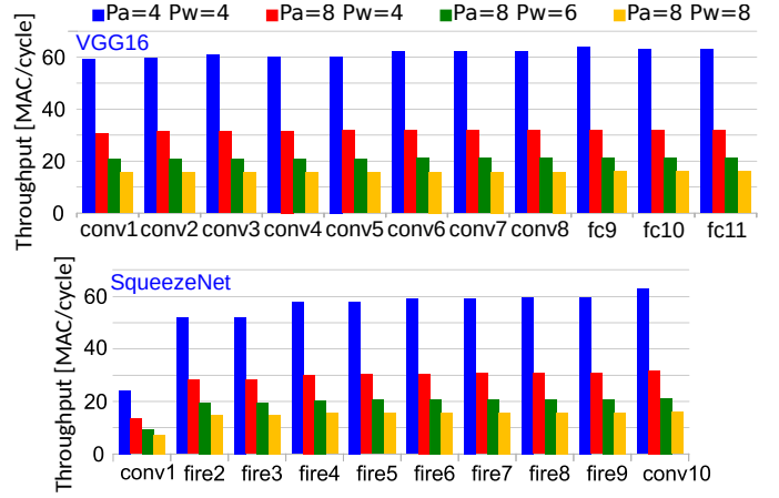
Fig. 4. Layers throughput over several bitwidth combinations.
