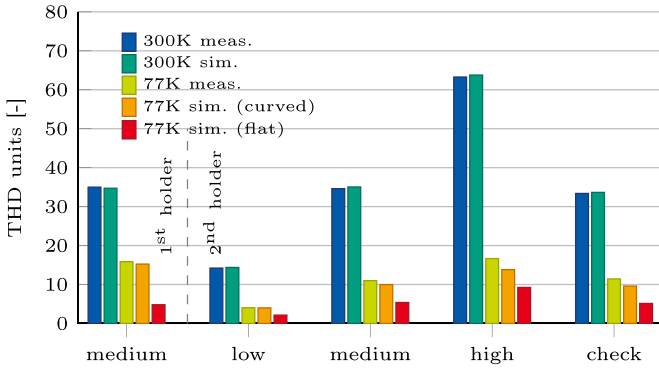
Figure 16. Measured and simulated magnetic field quality, given in units as a THD factor. Results are shown for four different positions of the iron bars. The field error is shown for both the iron bars alone, and with the HALO. Simulation results are also shown for HTS screens with flat geometry.
