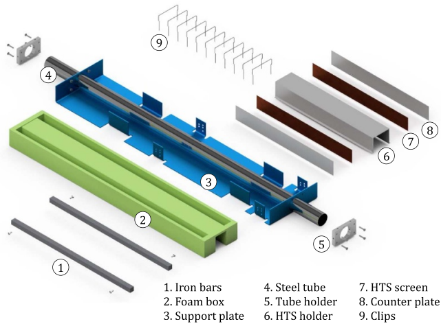
Figure 3. Exploded view of the parts of the experimental assembly. (1) Iron bars, (2) polyme foam box, (3) aluminum support plate, (4) stainless steel tube, (5) aluminum collars, (6) aluminum HTS holder, (7) HTS screens, (8) aluminum counter plates, (9) stainless steel clips.
