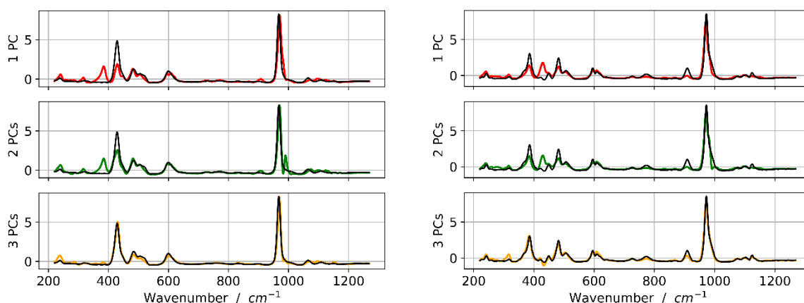
Figure 3 Reconstruction of two spectra (R060090 on the left and R100199 on the right) using an increasing number of PCs. Original spectrum is represented in black, colored lines are used for the model; it is possible to see how the addition of PCs improves the goodness of fit. Samples names stand for the spectra Rruff ID.
