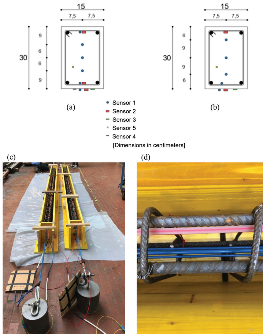
Fig. 8—FOS arrangement in cross sections: (a) Beam 1; and (b) Beam 2; (c) beam preparation with formwork; and (d) top view detail of longitudinal and transversal reinforcements with embedded FOSs.
