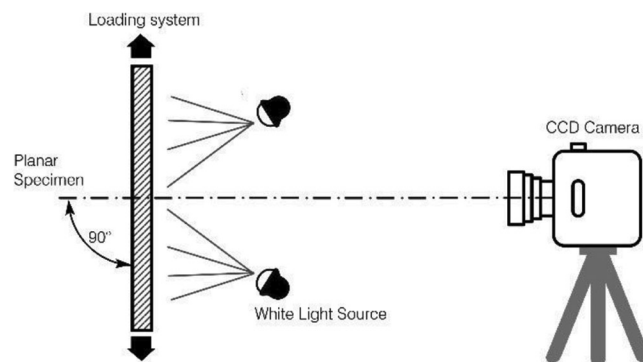
Fig. 1—Experimental setup for 2-D DIC.
