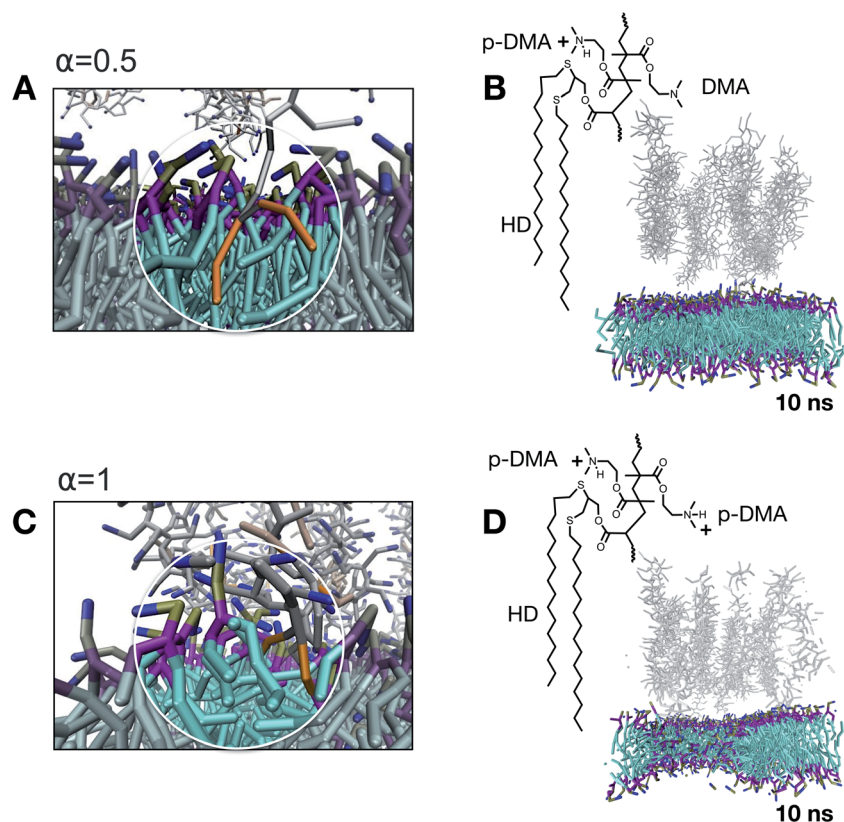
Fig. 5 Mechanistic insights into the first contact between the probe and lipid bilayer mediated by nonspecific interactions. Close-up snapshot for \alpha = 0.5 (A) highlighting the lipid extraction coupled with hydrophobic chain protrusion. Lipid membrane structural evolution after 10 ns of simulated evolution confirming the preservation of the structural integrity upon interaction (B). Close-up snapshot for \alpha = 1 (C) highlighting hydrophobic chain protrusion associated with unbalanced lipid extraction. Lipid membrane structural evolution after 10 ns of simulated evolution showing major changes in the membrane integrity upon interaction (D).
