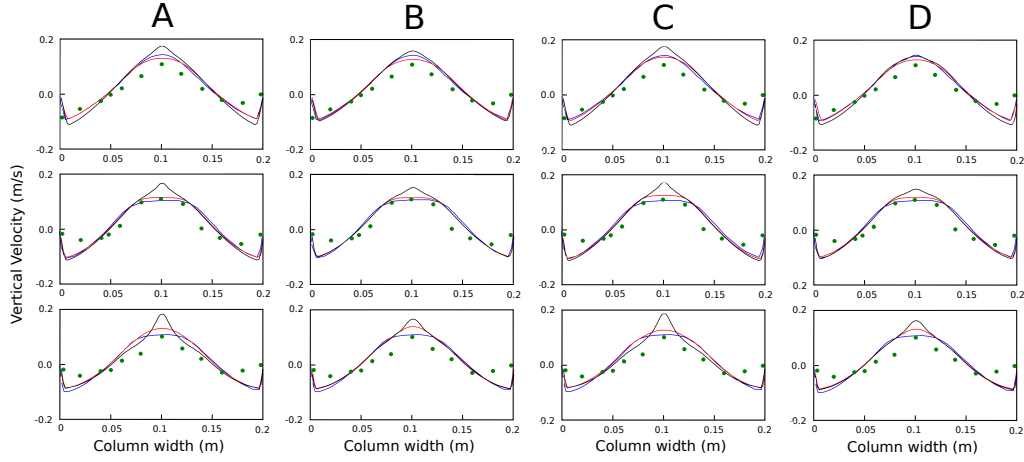
Figure 10: Comparison between experimental data, TFM and DMM at three different heights of the column studied by Pfleger and coworkers (from top to bottom: 0.37 cm - 0.25 cm - 0.13 cm). From left to right simulations obtained with the different simplifications are reported (A, B, C and D, respectively). The green circles represent the experimental data, whereas blue, black and red lines are the predictions obtained with TFM and DMM with options 1 and 2, respectively. WHAT SUPERFICIAL VELOCITY?
