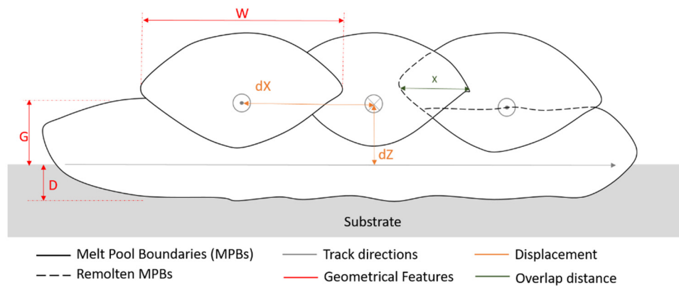
Figure 3. Schematic representation of two LP-DED layers build with no growth overlap and the 0/90° scanning strategy with bidirectional scanning in each layer.
