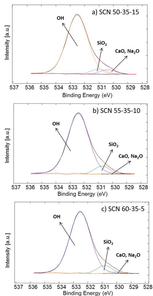
Figure 2. XPS high-resolution spectra (O region).
